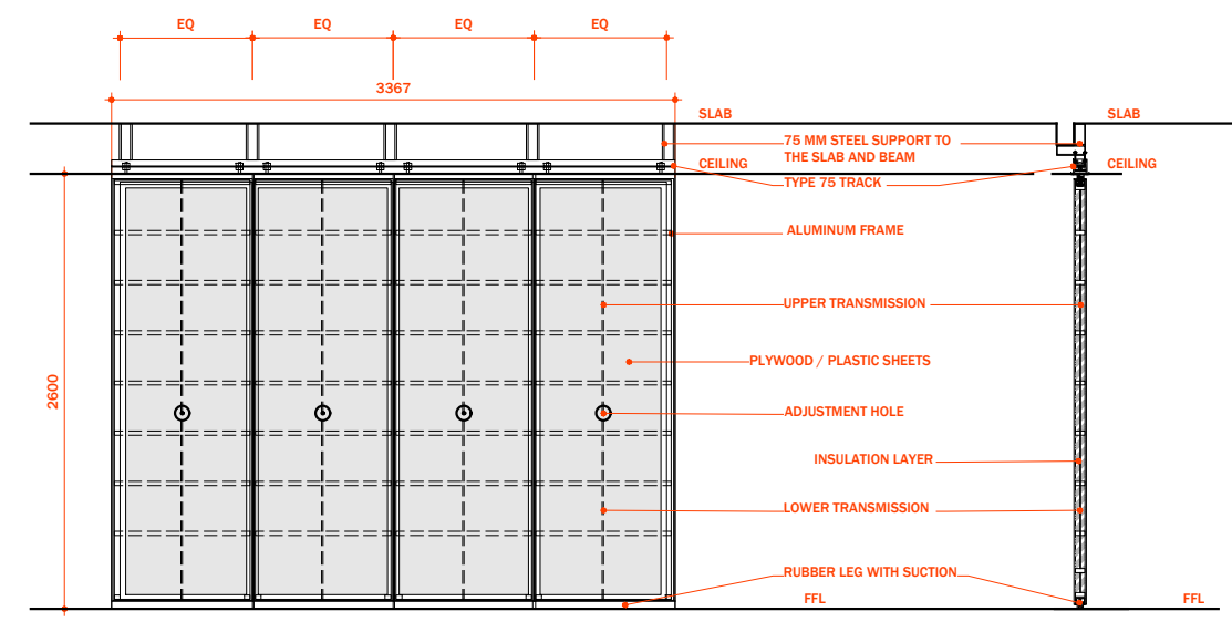
1 FOLDING SLIDING DOOR DETAIL 1 SCALE: 1:50
